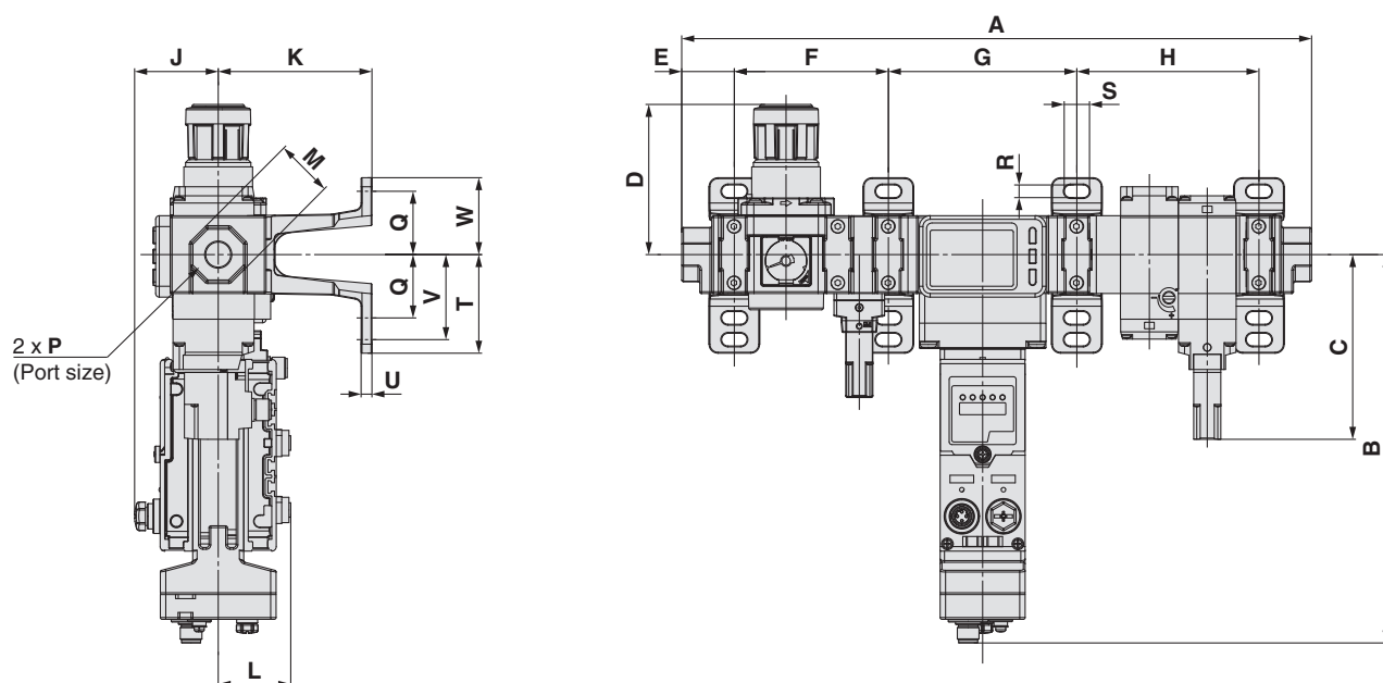
AMS20/30/40/60B-00D
