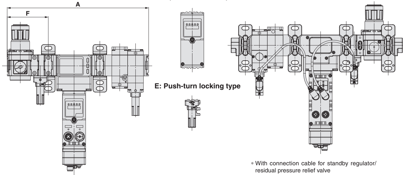
AMS20/30/40/60B-00D
